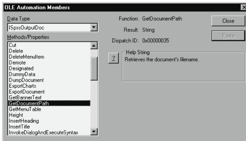
Figure 48-13 Object browser
