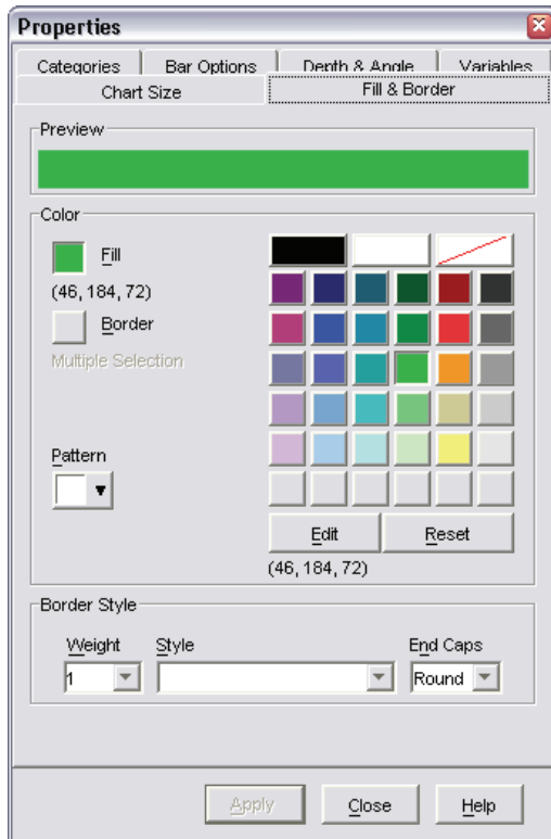
Figure 43-6 Properties window
