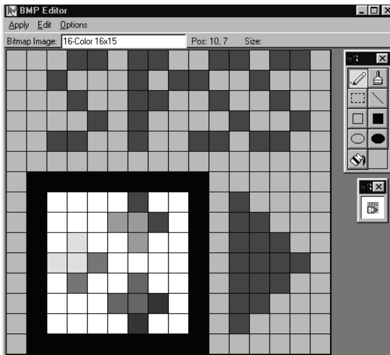
Figure 46-6 Bitmap Editor
