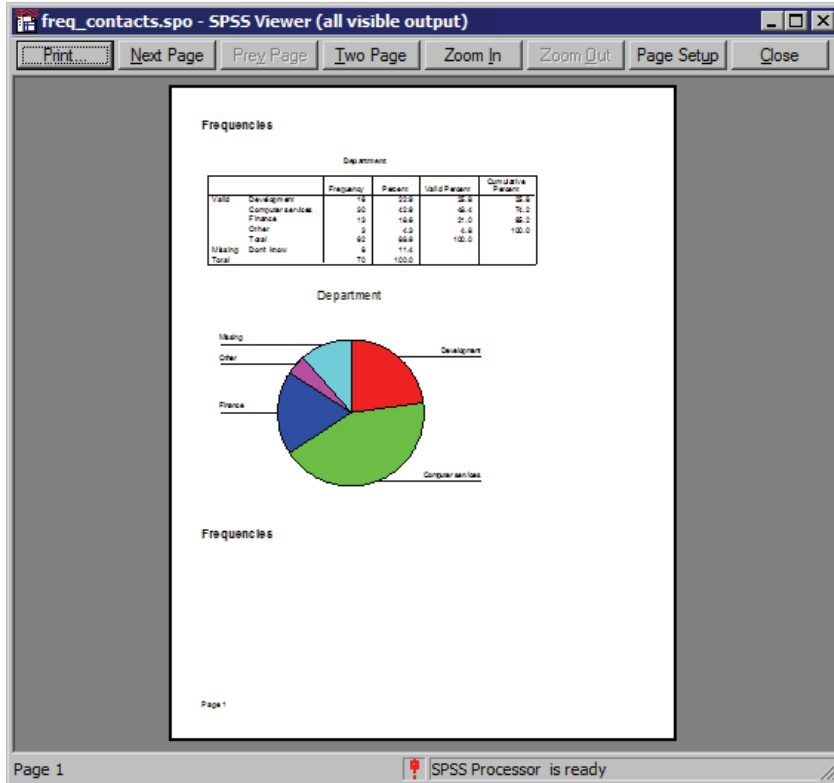
Figure 10-11 Print Preview
